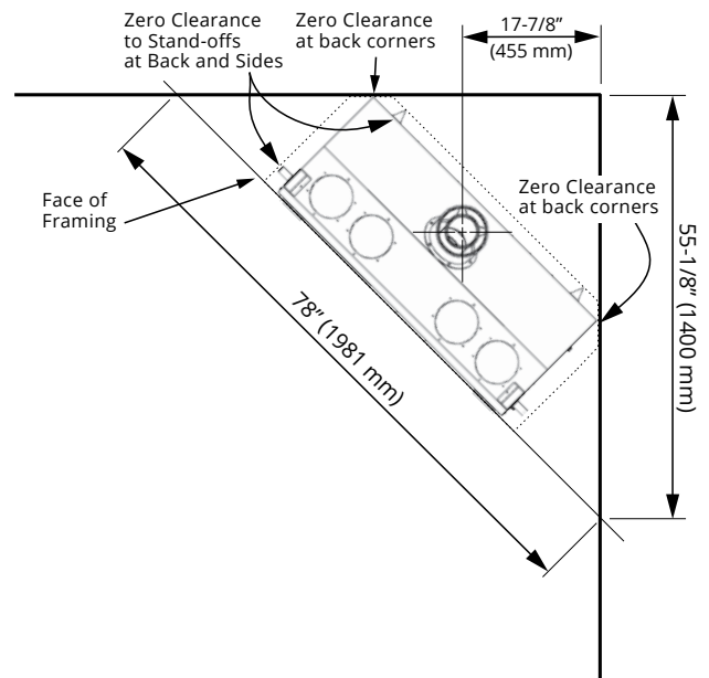
CORNER VIEW
