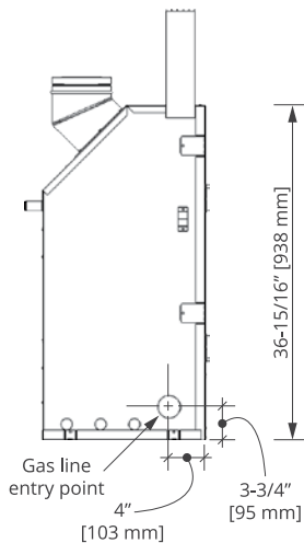
LEFT VIEW
