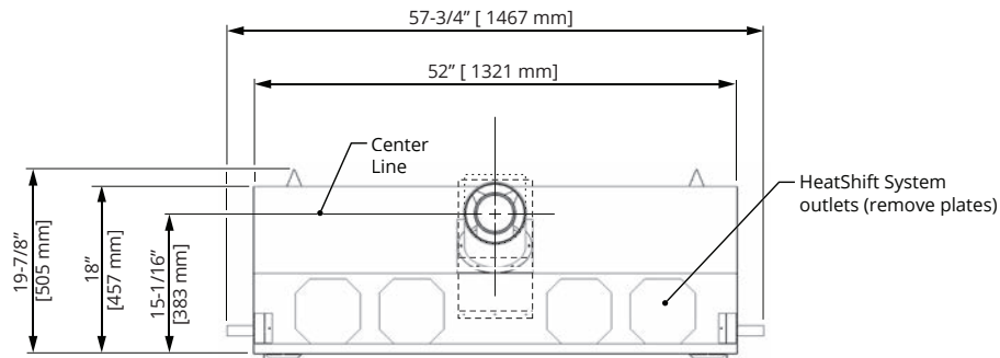
Top View
