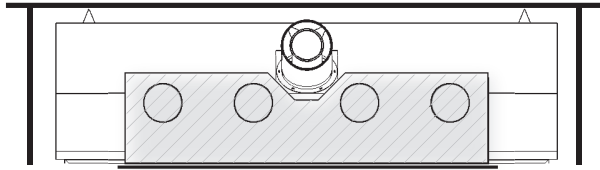
Front wall outlet using LDK1 or LDK4
