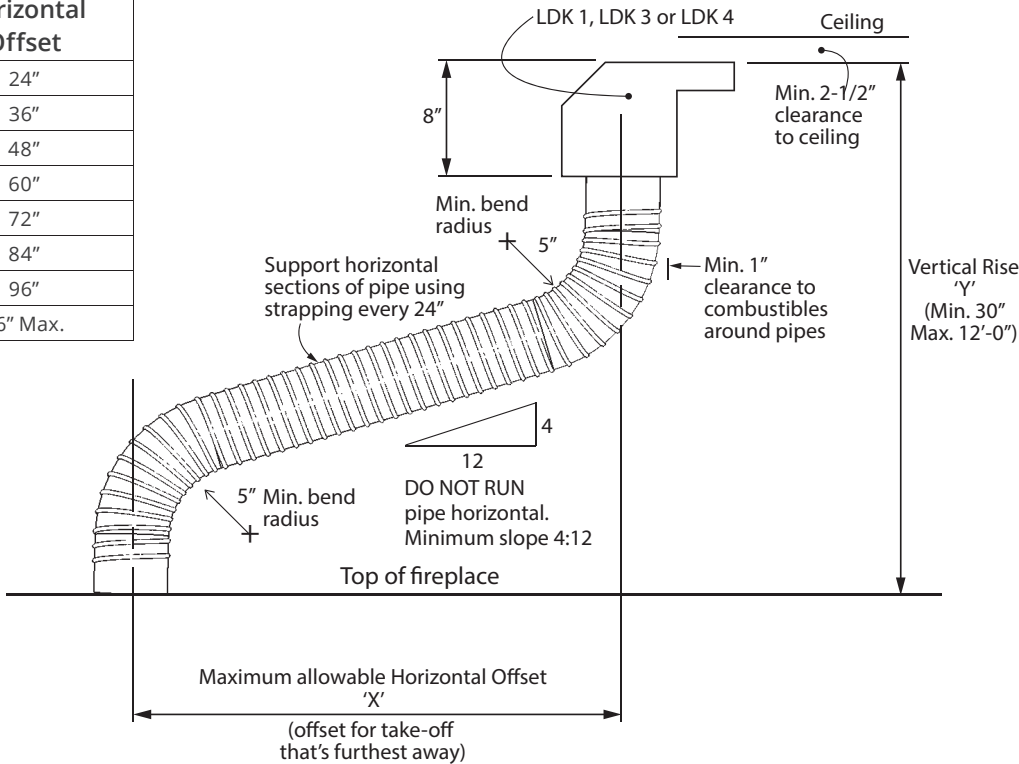
With Plenum
