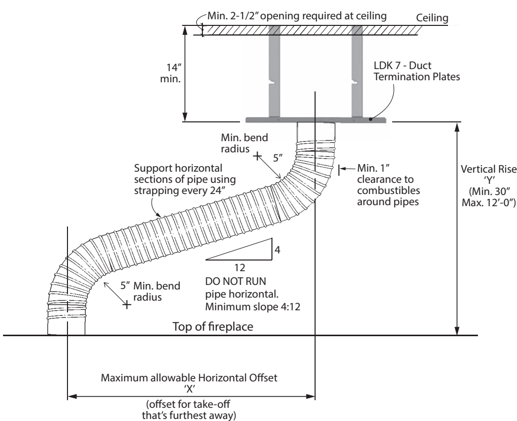
With Plates
