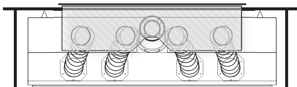
Rear wall outlet using LDK1 or LDK4 Note: Fireplace vent may conflict with plenum. Offset vent around plenum.
