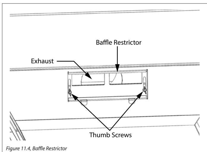
Figure 11.4, Baffle Restrictor
