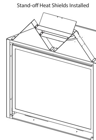
Figure 3.1, Stand-off Assembly and Installation
