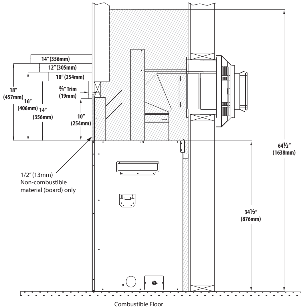
Figure 4.1, Combustible Mantel Requirements
